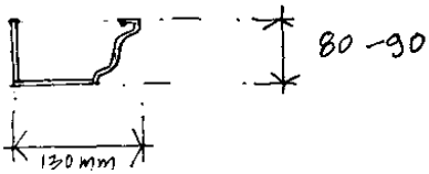
PERMITTED GUTTER PROFILES (IN CONTINUOUS ALUMINIUM TO COLOUR SPEC ONLY.)
