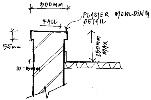
PARAPET CONDITION
