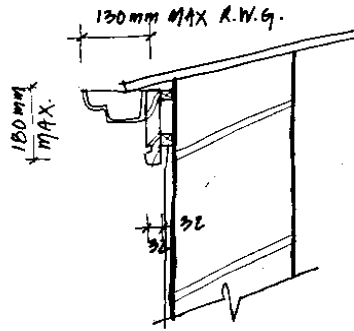
FASCIA CONDITIONS
